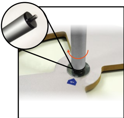
4. Screw the center pole into the internal thread of the base plate. Do not overtighten.
