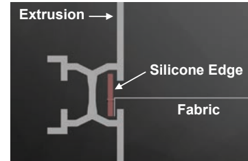
Cross section of extrusion channel with graphic installed
