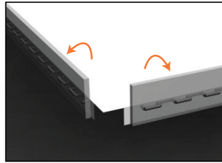
The silicone strips are rotated before being tucked into the channel.
