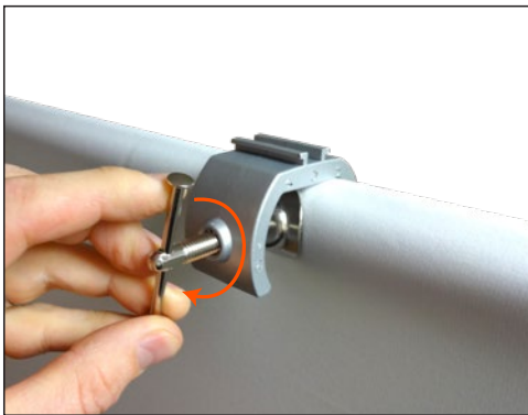
7. Attach optional light clamps to the top bar in desired locations. Tip: It is easier to do this before standing the display up.
