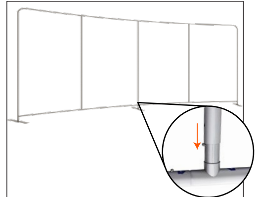
3. Assemble the frame by connecting the center support and all perimeter pieces of the frame.
